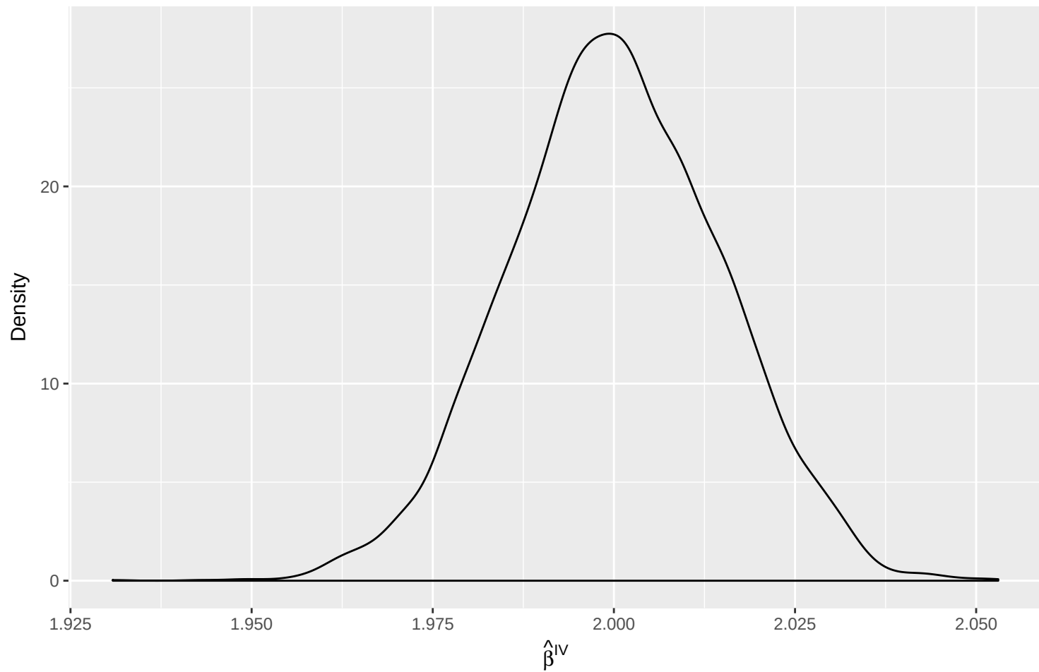
Density of IV Estimator with N = 10000 and \rho_{XZ} = .95
